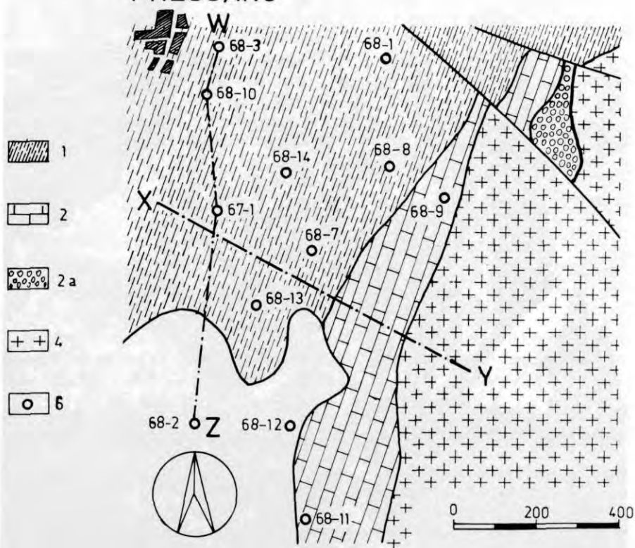
Fig. 5. Geological sketch map of the Lavís area
