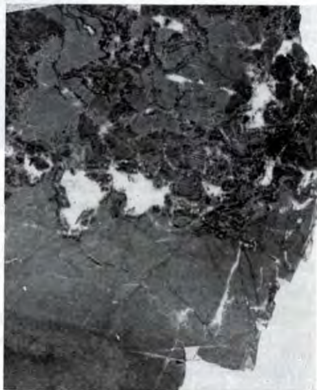
Fig. 4. Veinlet texture in part brecciated, of the sphalerite (sphaalenblende) in primary dolomite. Scale 1:1
