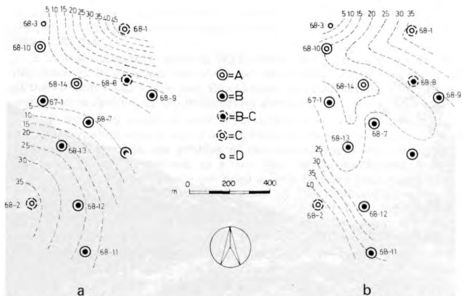
Fig. 7. Isopach maps of "Grödener sandstone" (a) and Bellerophon formation (b) in the Lavis area
